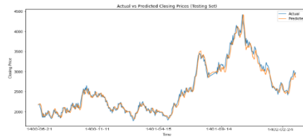
The proposed LSTM-CNN Without PSO
